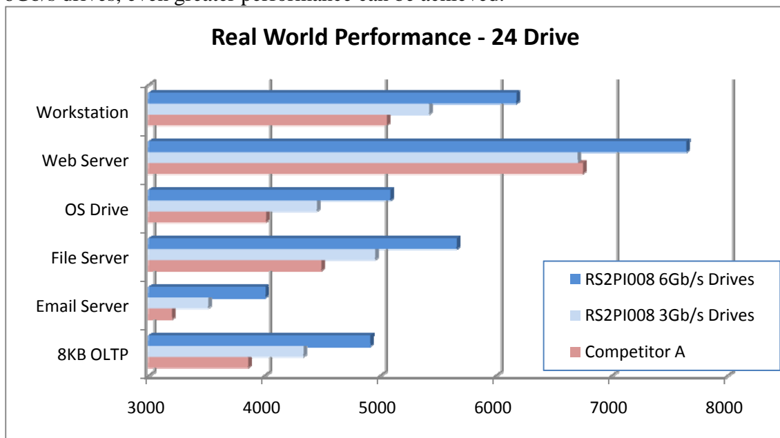
Figure 3 - Competitive real-world workload performance comparison for Intel RAID RS2PI008 controller and Competitor A using twenty-four 15k SAS drives in a RAID 5 array.
