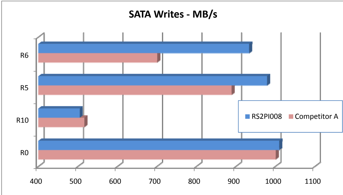
Figure 1 – Competitive performance analysis for controllers with 24 3Gb/s 7200 RPM SATA hard drives in write-intensive environments
