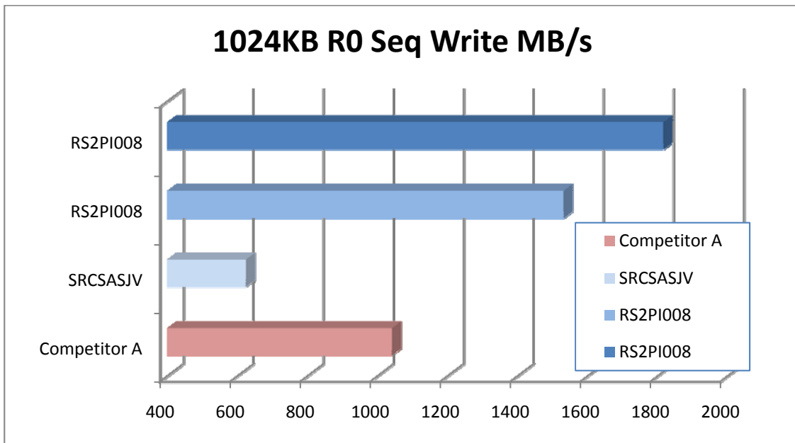
Figure 6 – RAID 0 Sequential Write Workload with Write Back Cache Enabled using 24 SAS Drives
